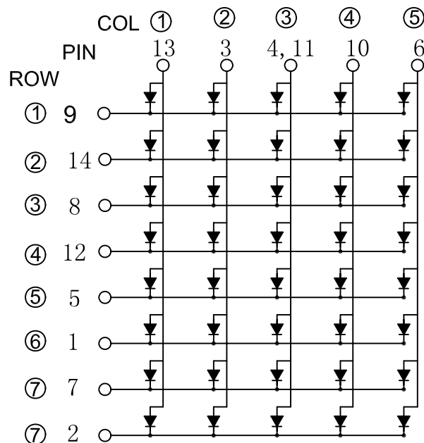
COMMON CATHODE
