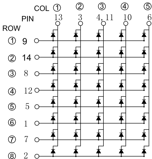
COMMON ANODE
