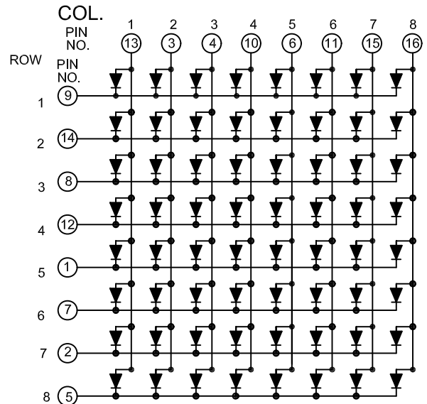
COMMON CATHODE
